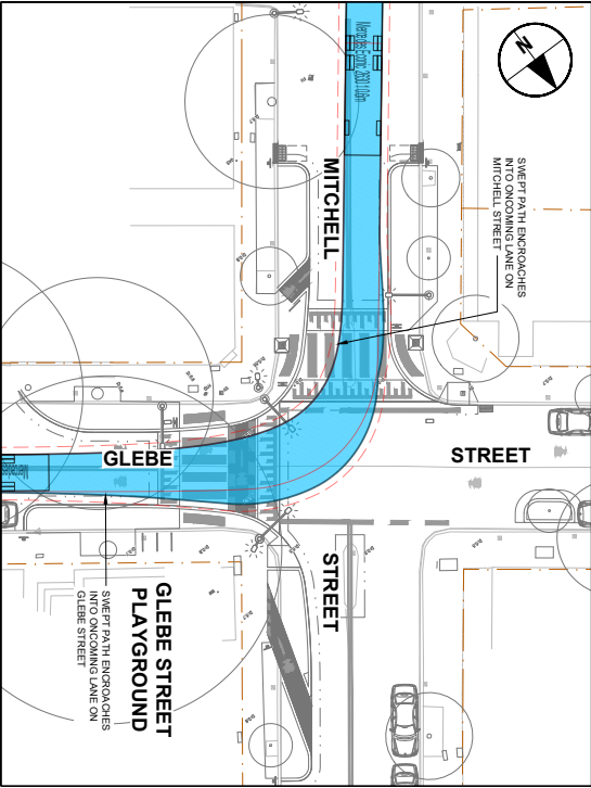
10.6m GARBAGE TRUCK TURNING RIGHT FROM MITCHELL STREET (SOUTH) TO GLEBE STREET SCALE 1:200
