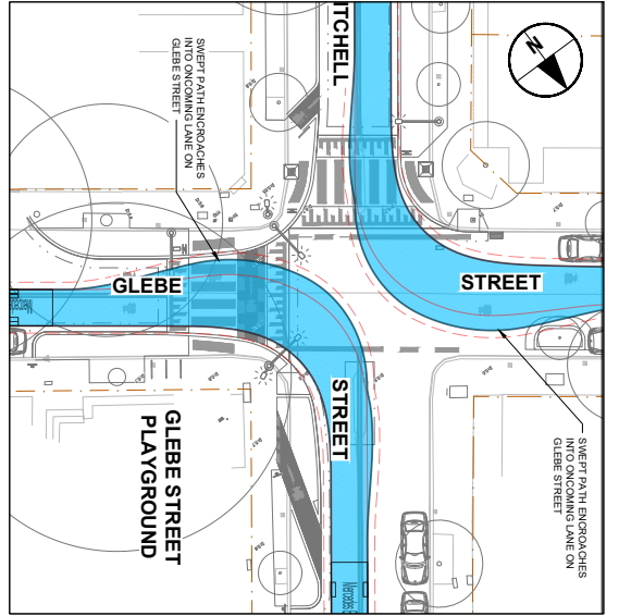
10.6m GARBAGE TRUCK LEFT TURNS ONLY SCALE 1:200
