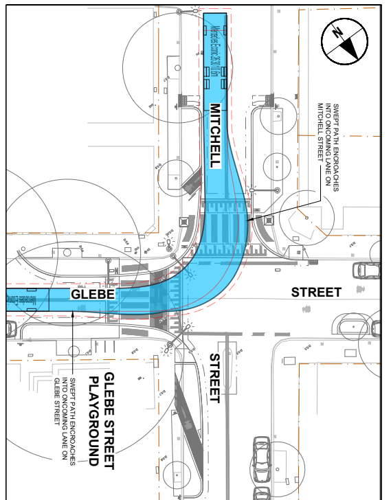
10.6m GARBAGE TRUCK TURNING LEFT FROM GLEBE STREET (EAST) ONTO MITCHELL STREET SCALE 1:200
