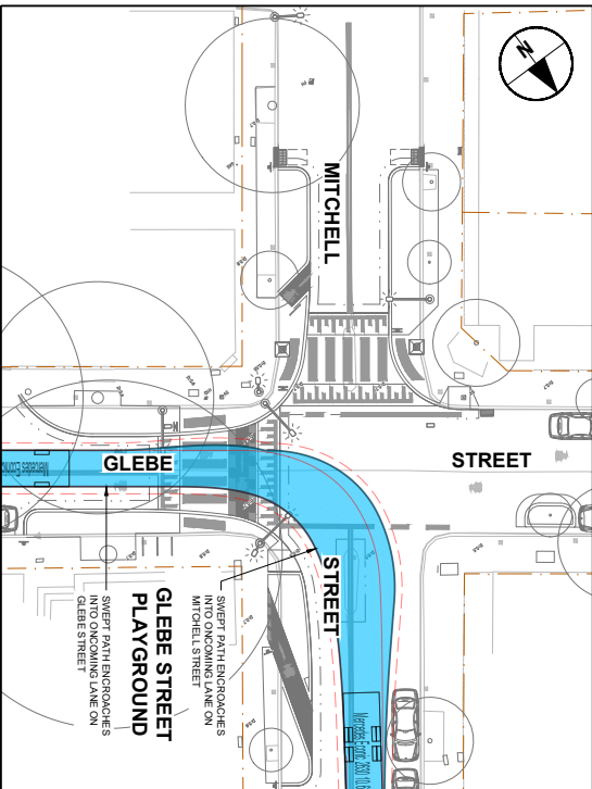
10.6m GARBAGE TRUCK TURNING RIGHT FROM GLEBE STREET (EAST) TO MITCHELL STREET SCALE 1:200
